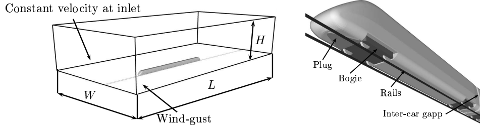
Figure 1: a) Geometry of the computational domain of the high-speed train leaving the tunnel. b) Part of the geometry of the train showing the loco from below.
