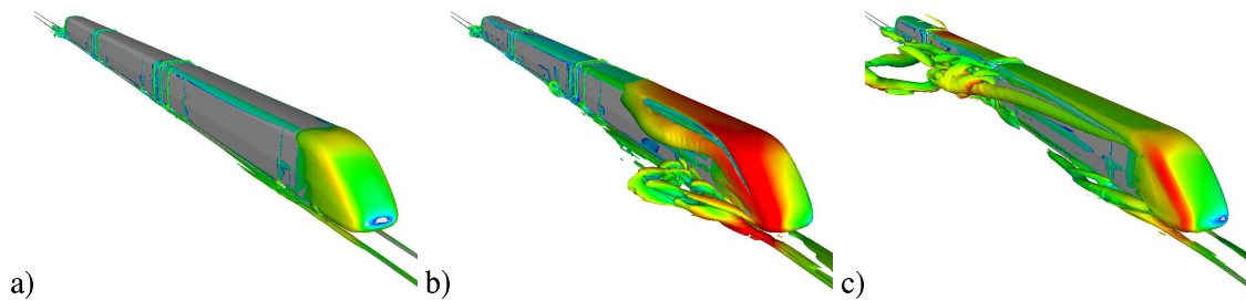
Figure 2: An isosurface of the second invariant of the velocity gradient colored with velocity magnitude. Figure a) shows the flow at the time when the wind gust has reached the train. The time difference between two pictures is 0.72s.
